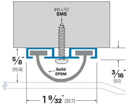
#952 Aluminum
