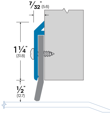
#950 Aluminum
