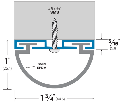
#972 Aluminum
